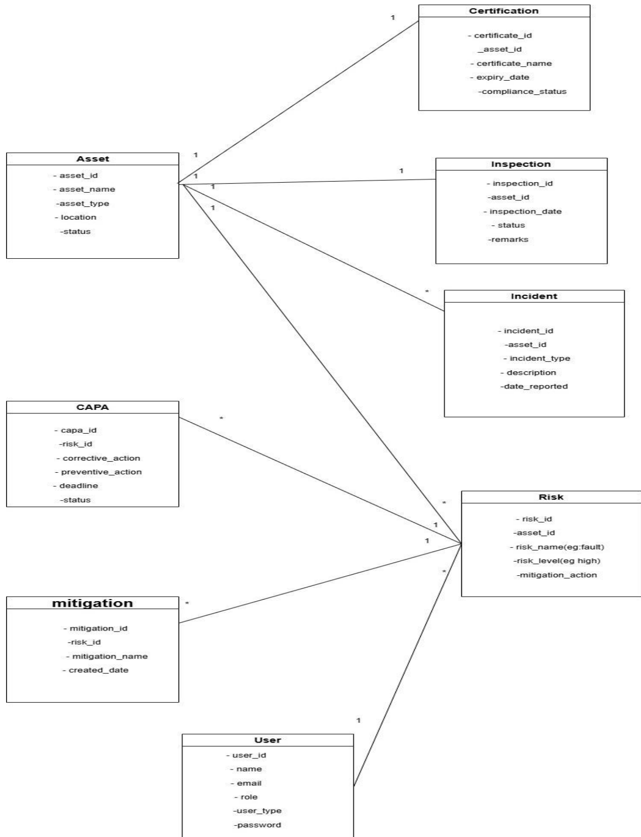
Figure 02: ERD diagram
